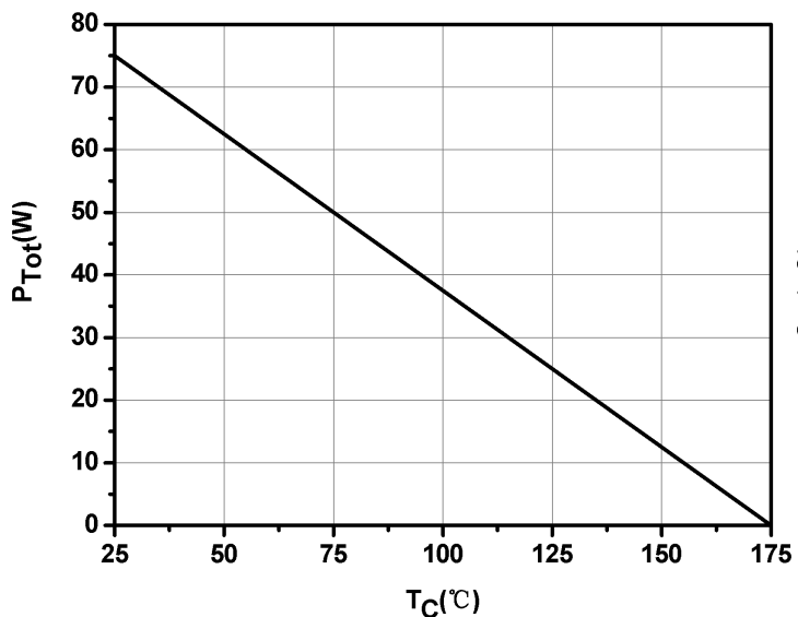
Fig.5-Power Derating
